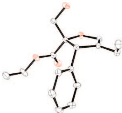
Figure 3. X-ray structure of isoxazoline 9 .
