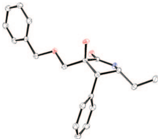
Figure 4. X-ray structure of lactam 11 .
