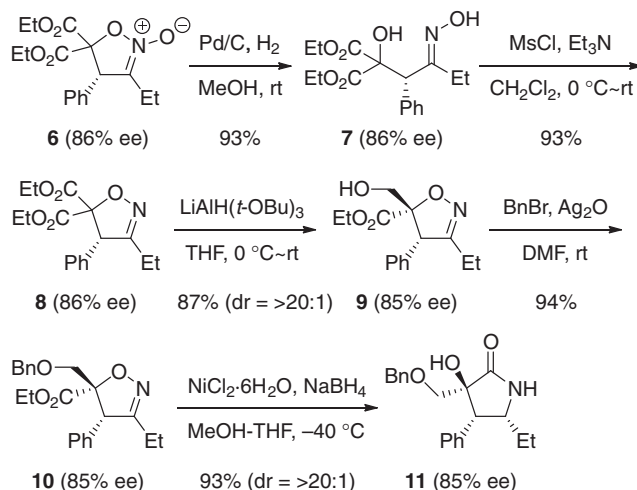
Scheme 3. Transformation of isoxazoline- N -oxide 6 .
