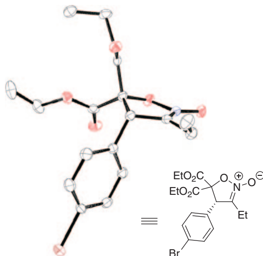
Figure 1. X-ray structure of isoxazoline- N -oxide.
