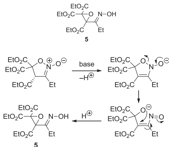
Scheme 2. A possible reaction pathway for the formation of oxime epoxide 5 .
