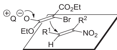
Figure 2. Plausible transition state model.
