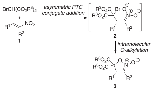
Scheme 1. Asymmetric synthesis of isoxazoline- N -oxides by asymmetric phase-transfer conjugate addition and intramolecular O -alkylation.
